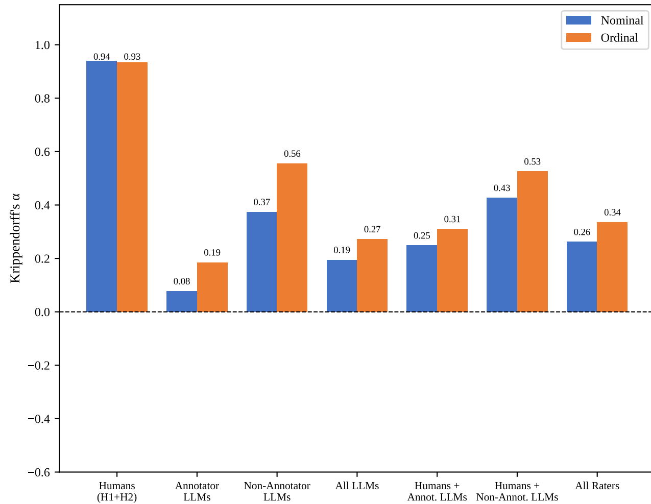
Span+Description (C2) Nominal vs Ordinal \alpha
