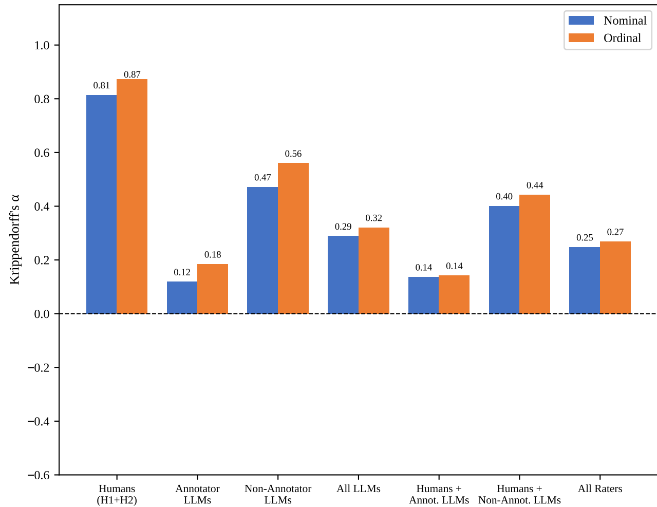
Correction (C4) Nominal vs Ordinal \alpha
