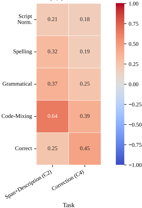
ICC(A,1) — All Raters
