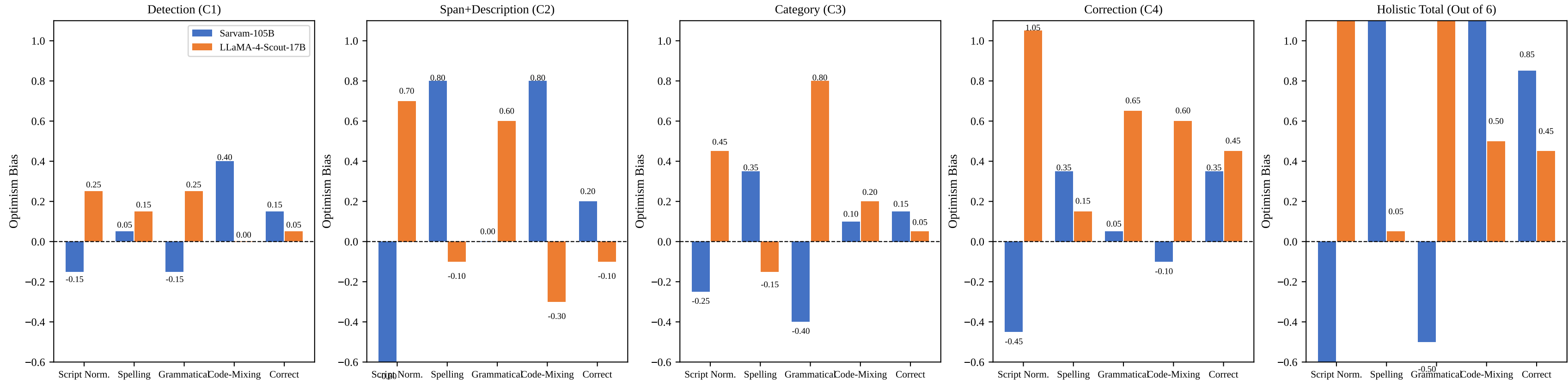
Optimism Bias of Self-Evaluating LLMs by Category and Task (positive = more lenient toward own outputs than human baseline)
