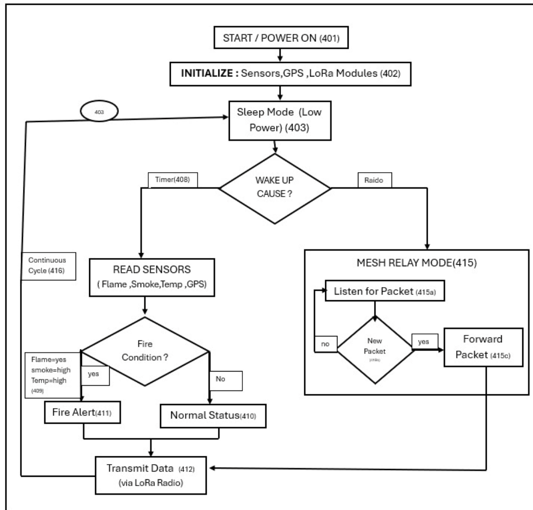
FIG .4 : Flowchart of Integrated Sensor Node Operation
