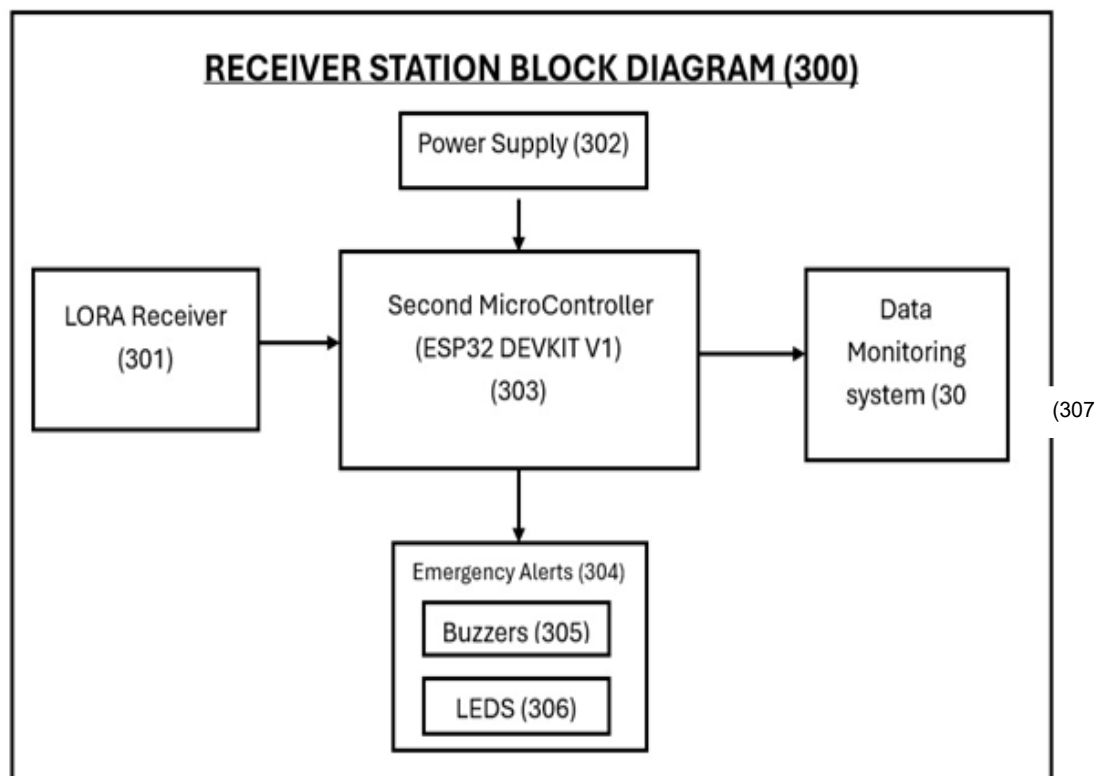
FIG .3 : Receiver/Base Station Block Diagram
