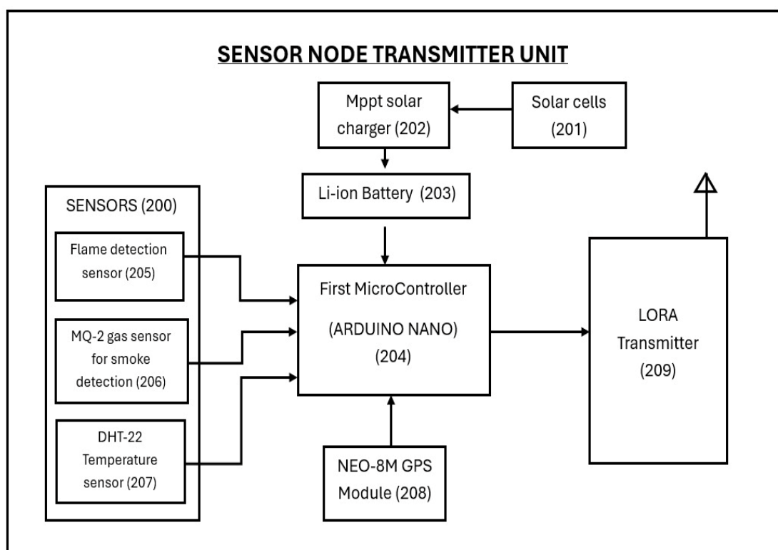
FIG.2 : Transmitter/Sensor Node Block Diagram
