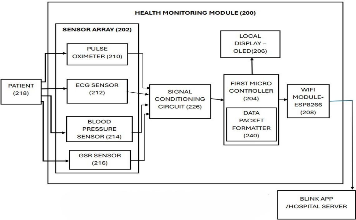
FIG2: HEALTH MONITORING MODULE(HMT)
