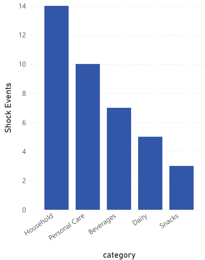
Shock Events by category
