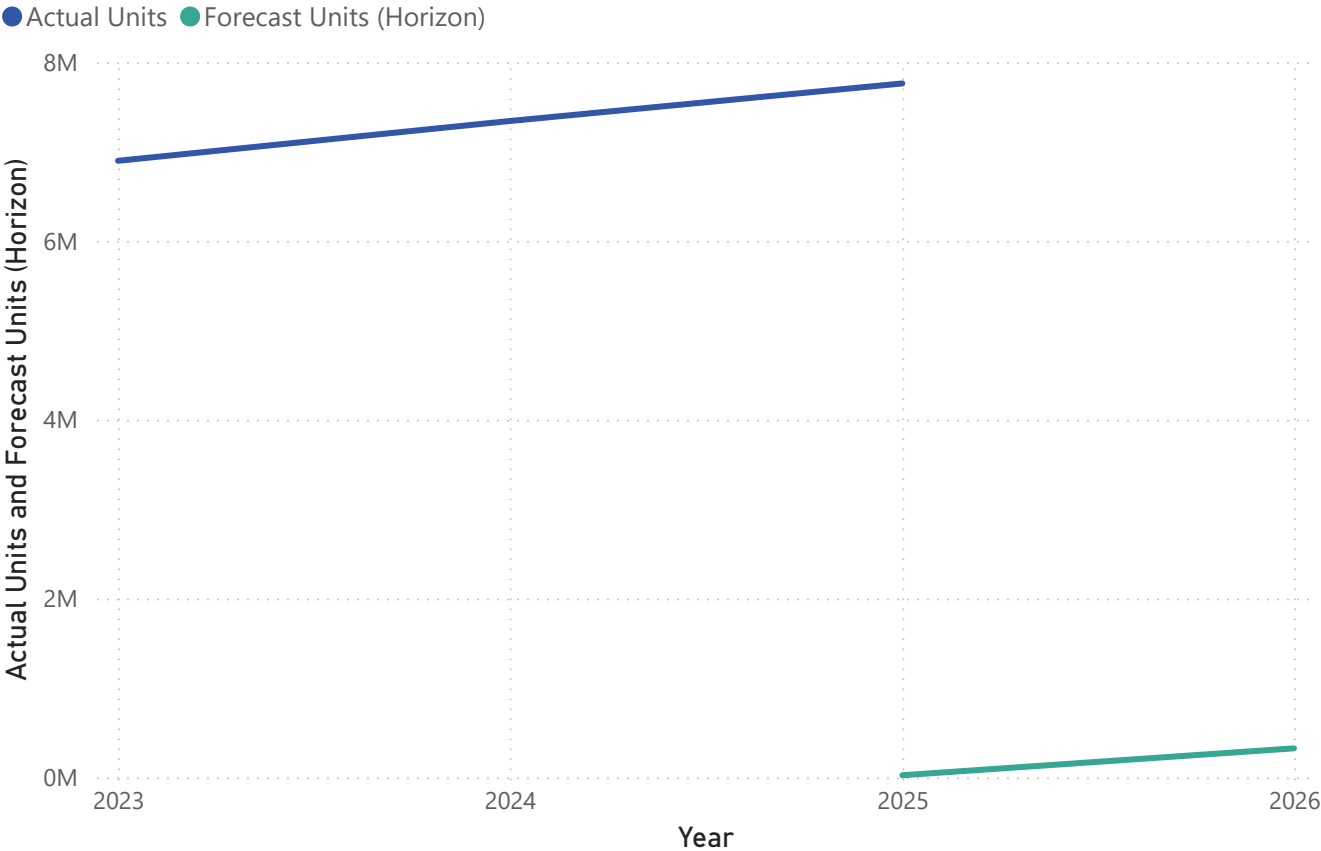
Actual Units and Forecast Units (Horizon) by Year
