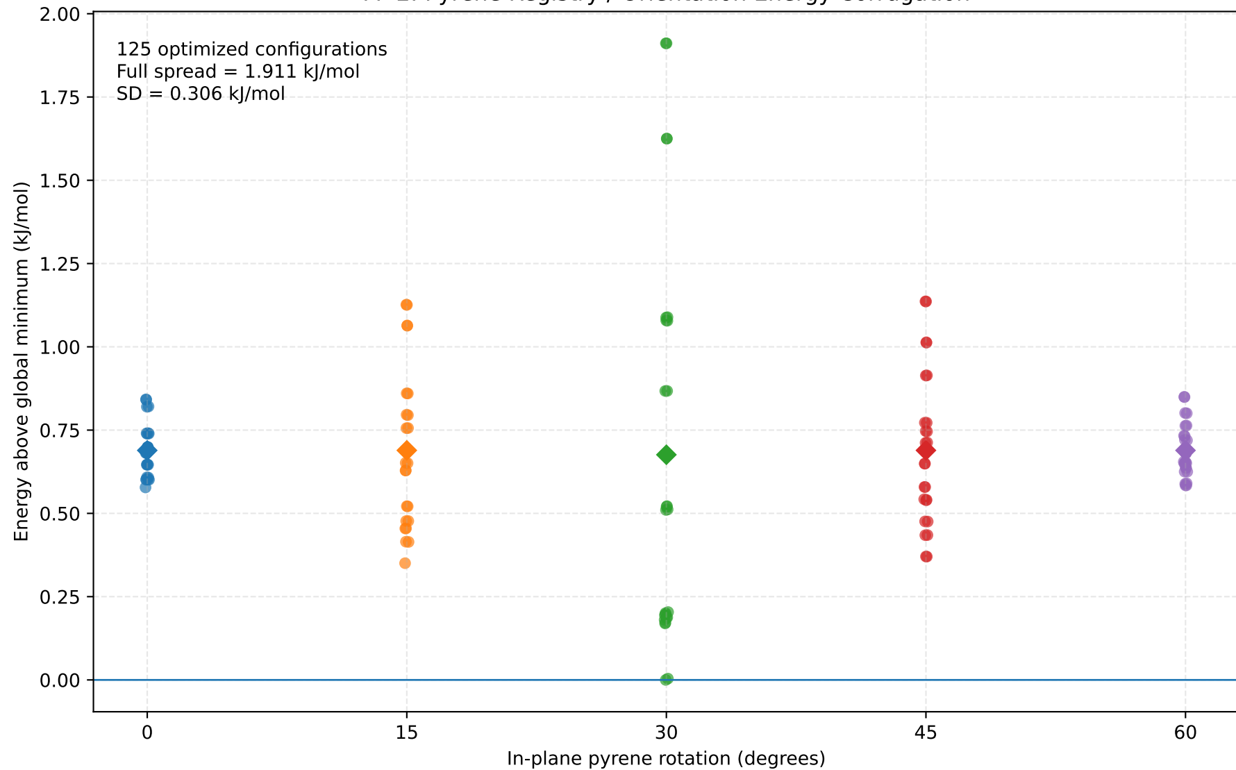
FF-2: Pyrene Registry / Orientation Energy Corrugation
