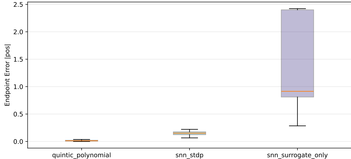
Endpoint Accuracy
