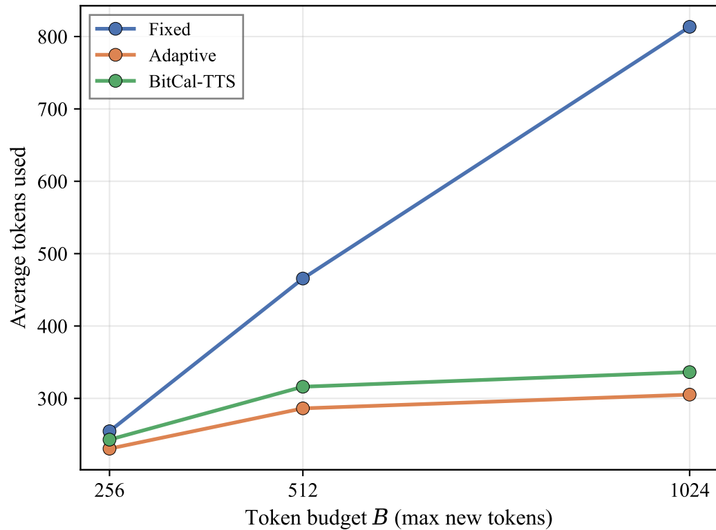
Qwen2.5-7B-Instruct (4-bit): compute vs budget
