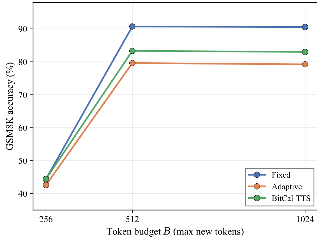
Qwen2.5-7B-Instruct (4-bit): accuracy vs budget
