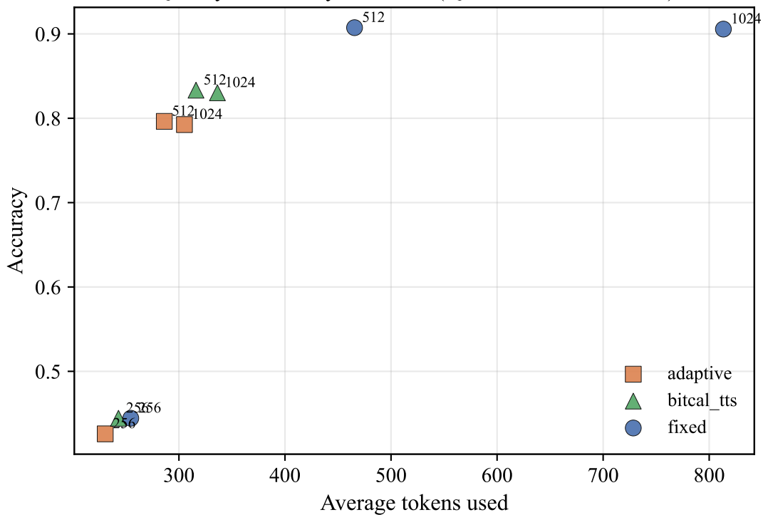
Quality–efficiency trade-off (Qwen2.5-7B, GSM8K)
