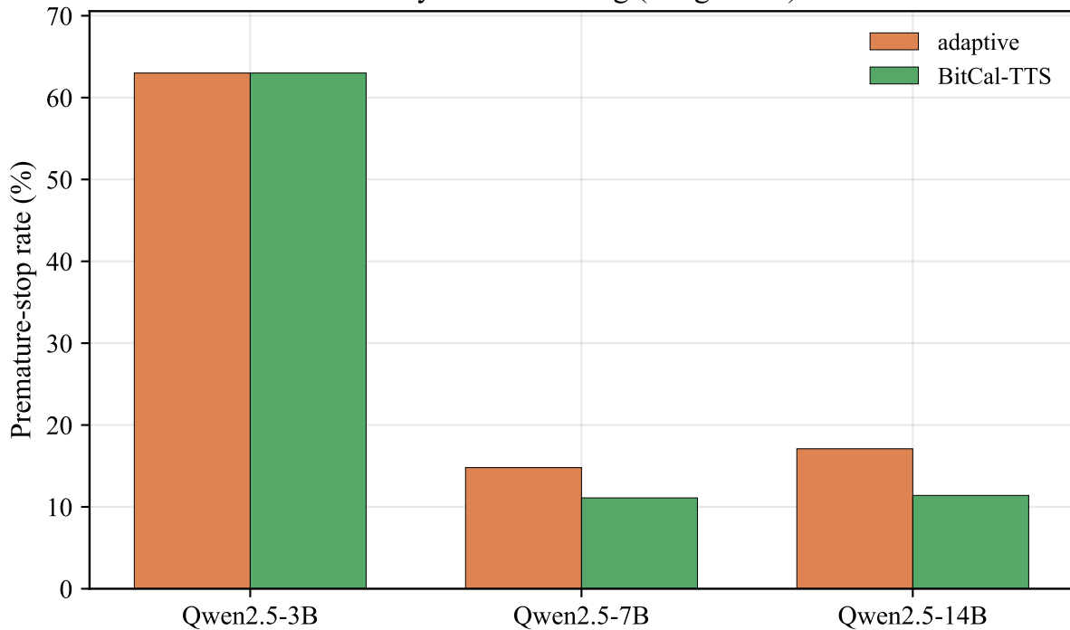
Early halt and wrong (budget 512)
