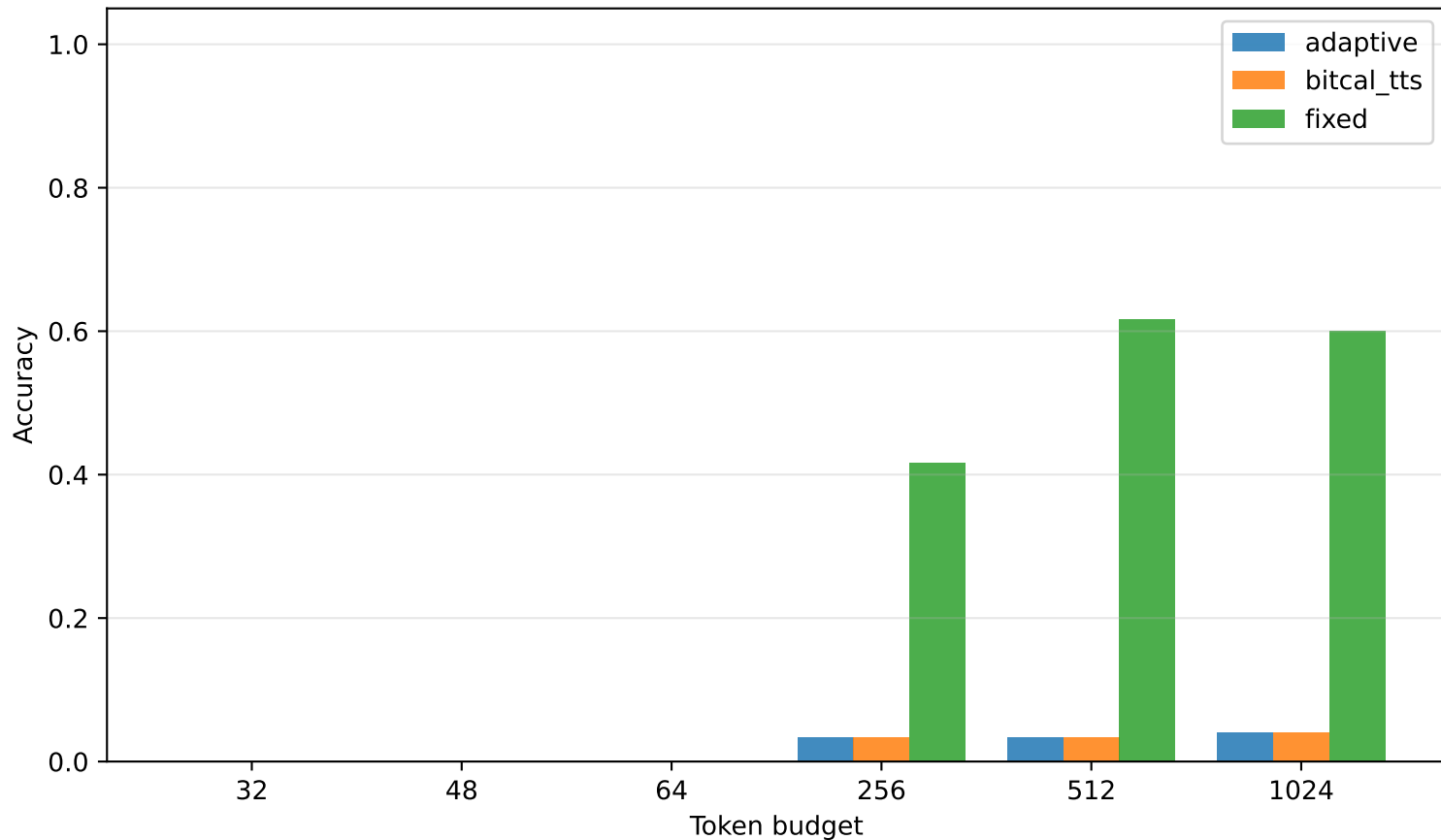
Accuracy by method and token budget
