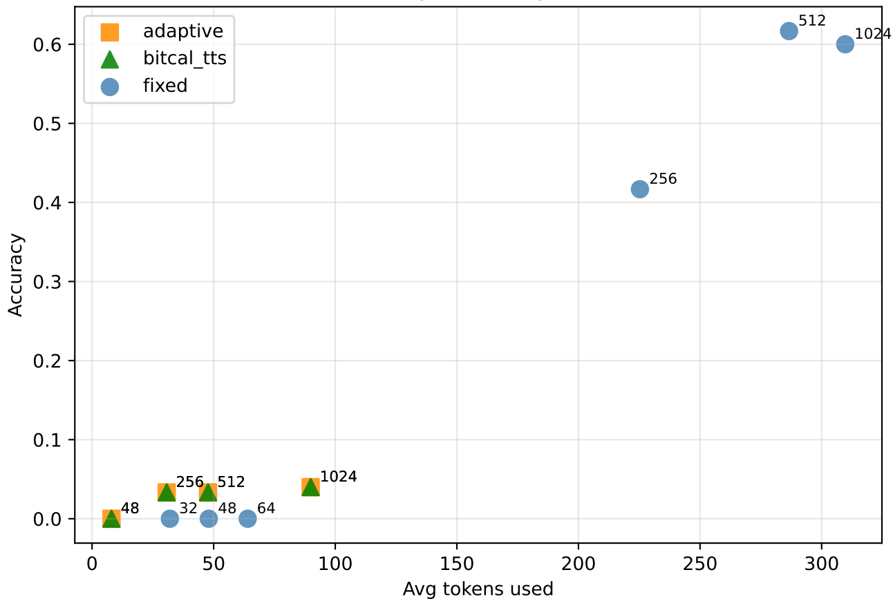
BitCal-TTS: Quality-Efficiency Pareto (GSM8K)
