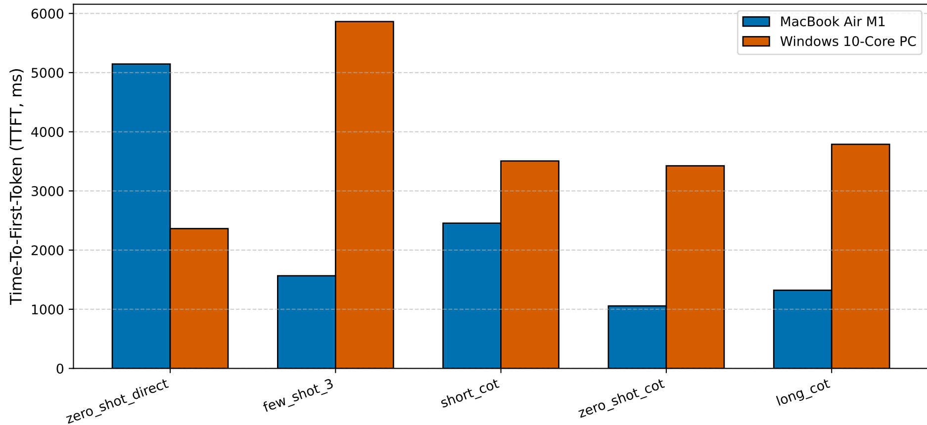
Time-To-First-Token by Hardware and Prompt Strategy
