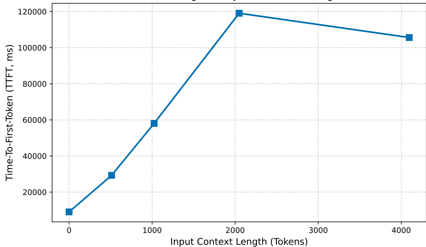
TTFT Scaling with Injected Context Length
