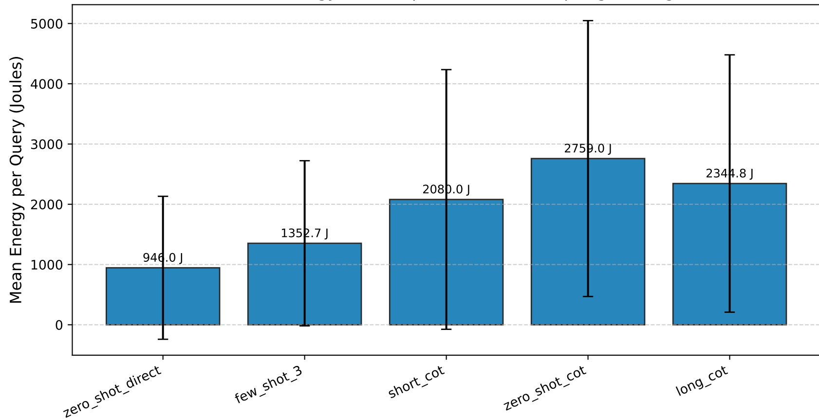
Inference Energy Consumption Across Prompting Strategies
