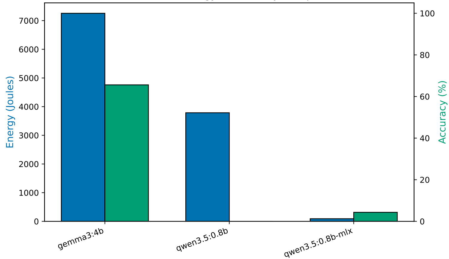
Cross-Model Energy & Accuracy Comparison
