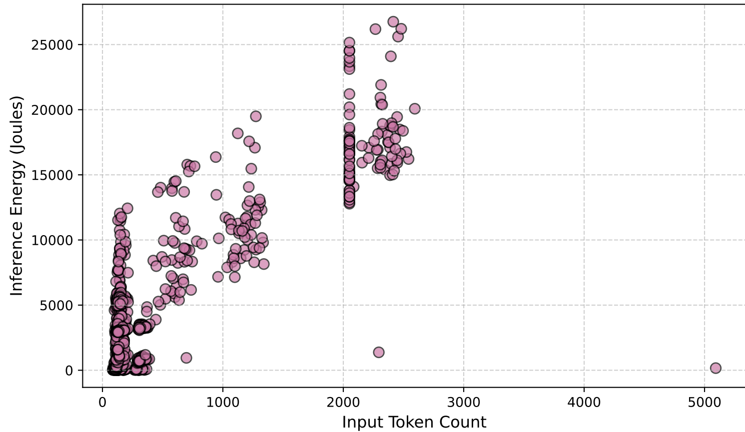
Input Token Load vs. Energy Expenditure
