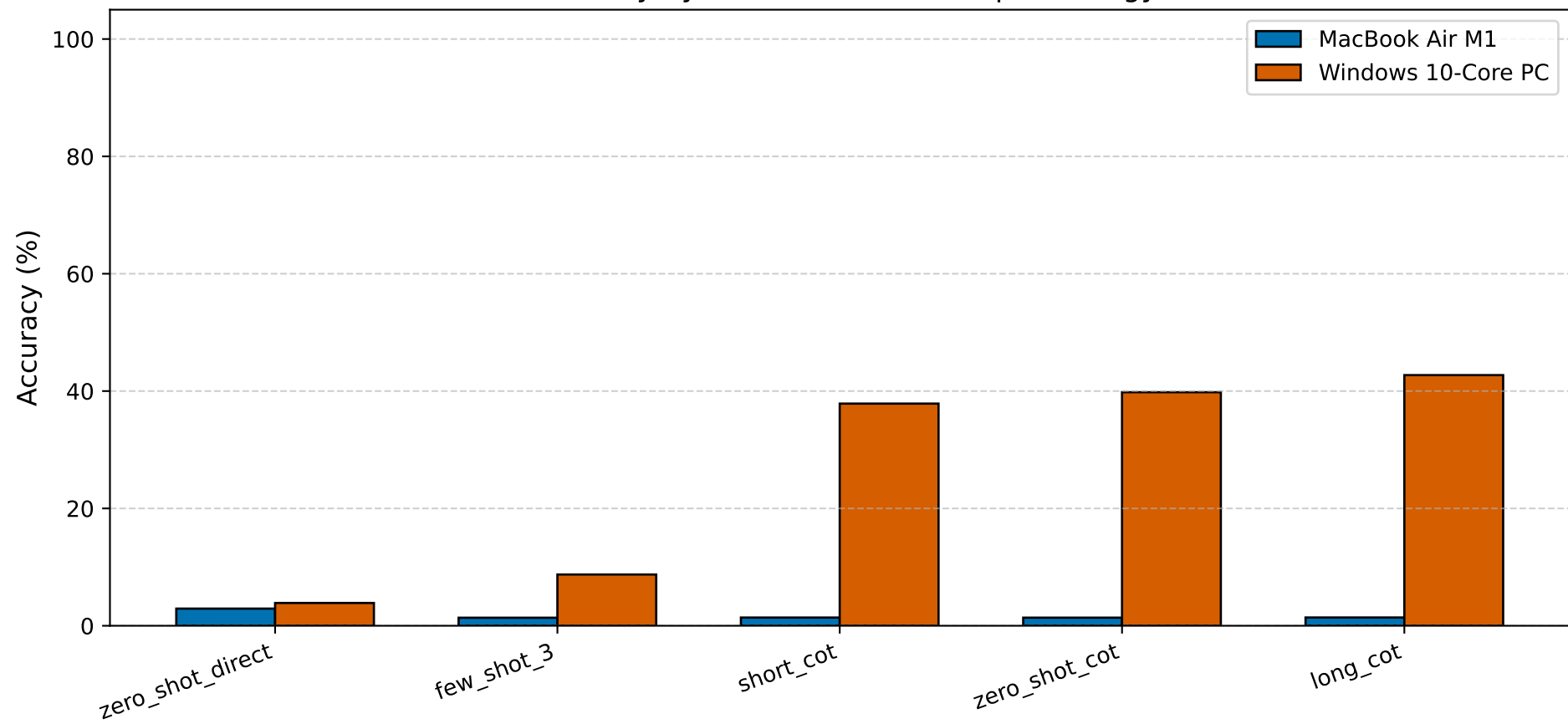
Accuracy by Hardware and Prompt Strategy
