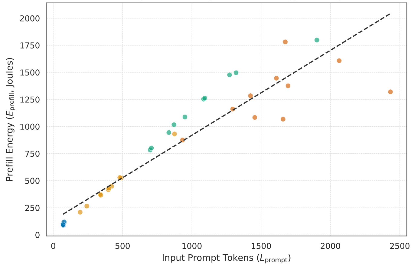
Prompt Processing (Prefill) Energy Scaling
