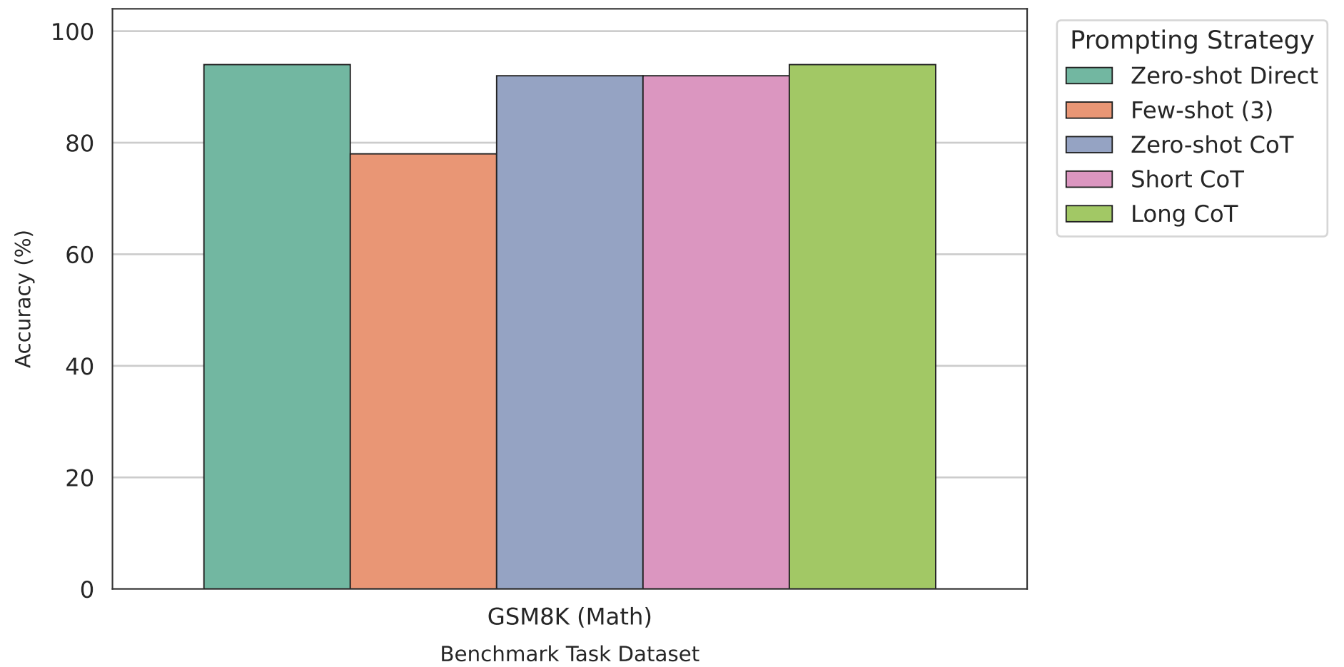
Task Accuracy by Prompting Strategy — Model: qwen3.5:9b (windows_10core_pc)
