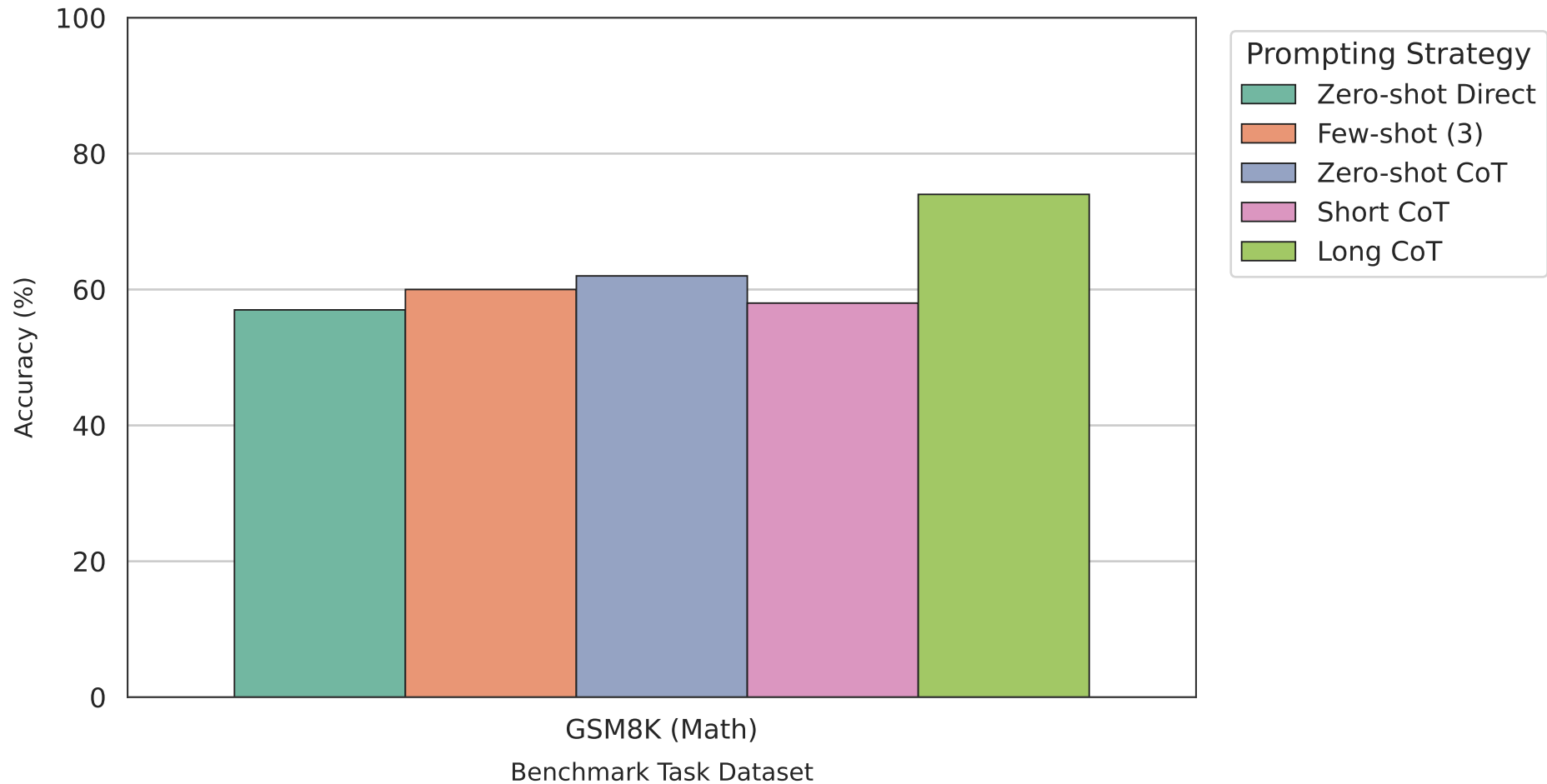
Task Accuracy by Prompting Strategy — Model: qwen3.5:2b-mlx (macbook_air_m1)
