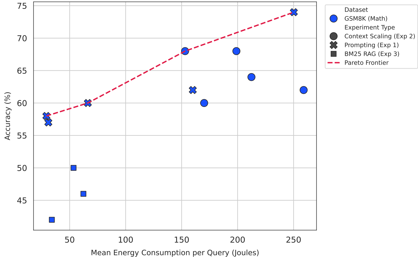
Energy vs. Accuracy Trade-Off & Pareto Frontier — qwen3.5:2b-mlx
