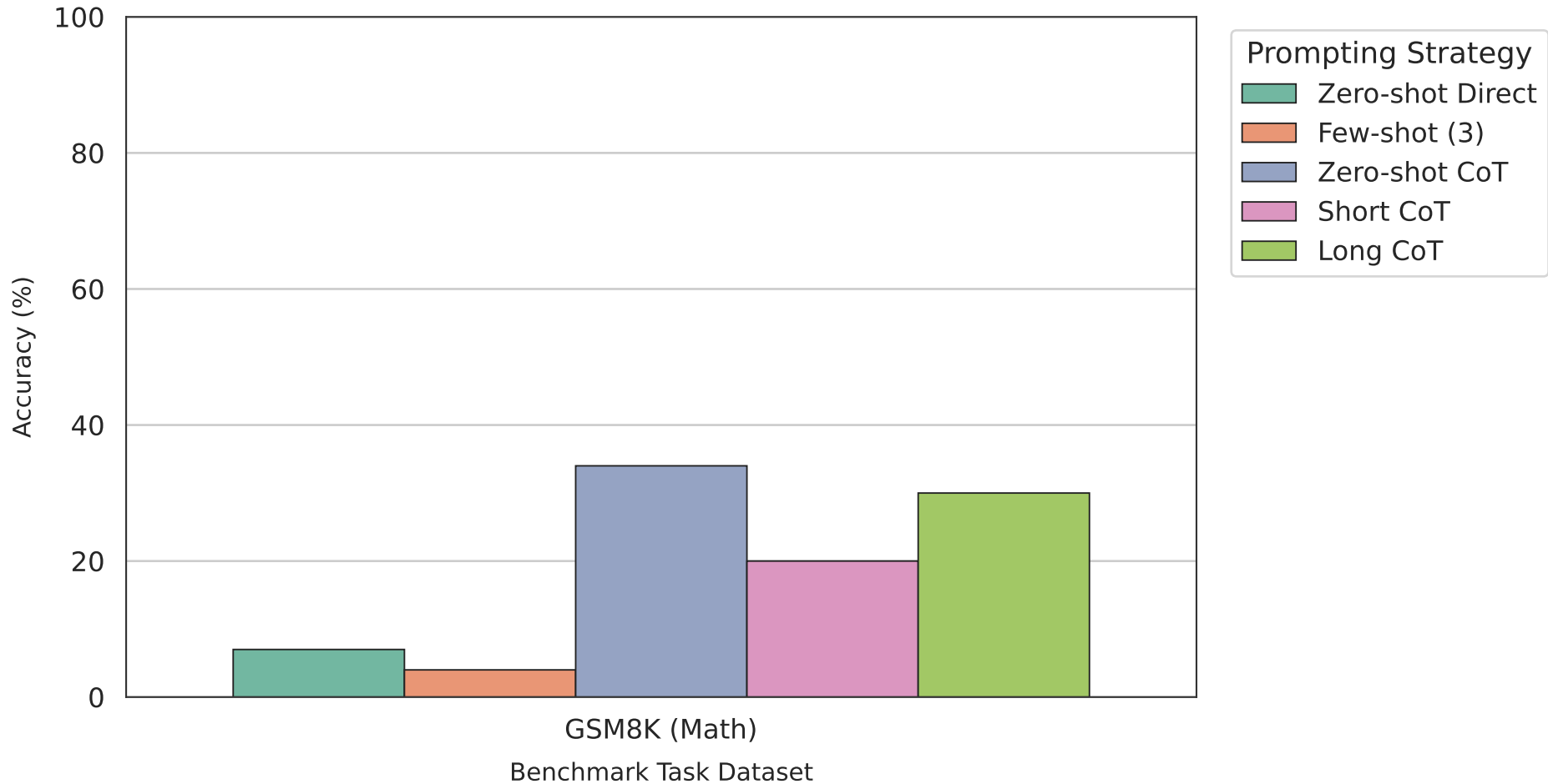
Task Accuracy by Prompting Strategy — Model: gemma3:1b (kaggle_t4_gpu)
