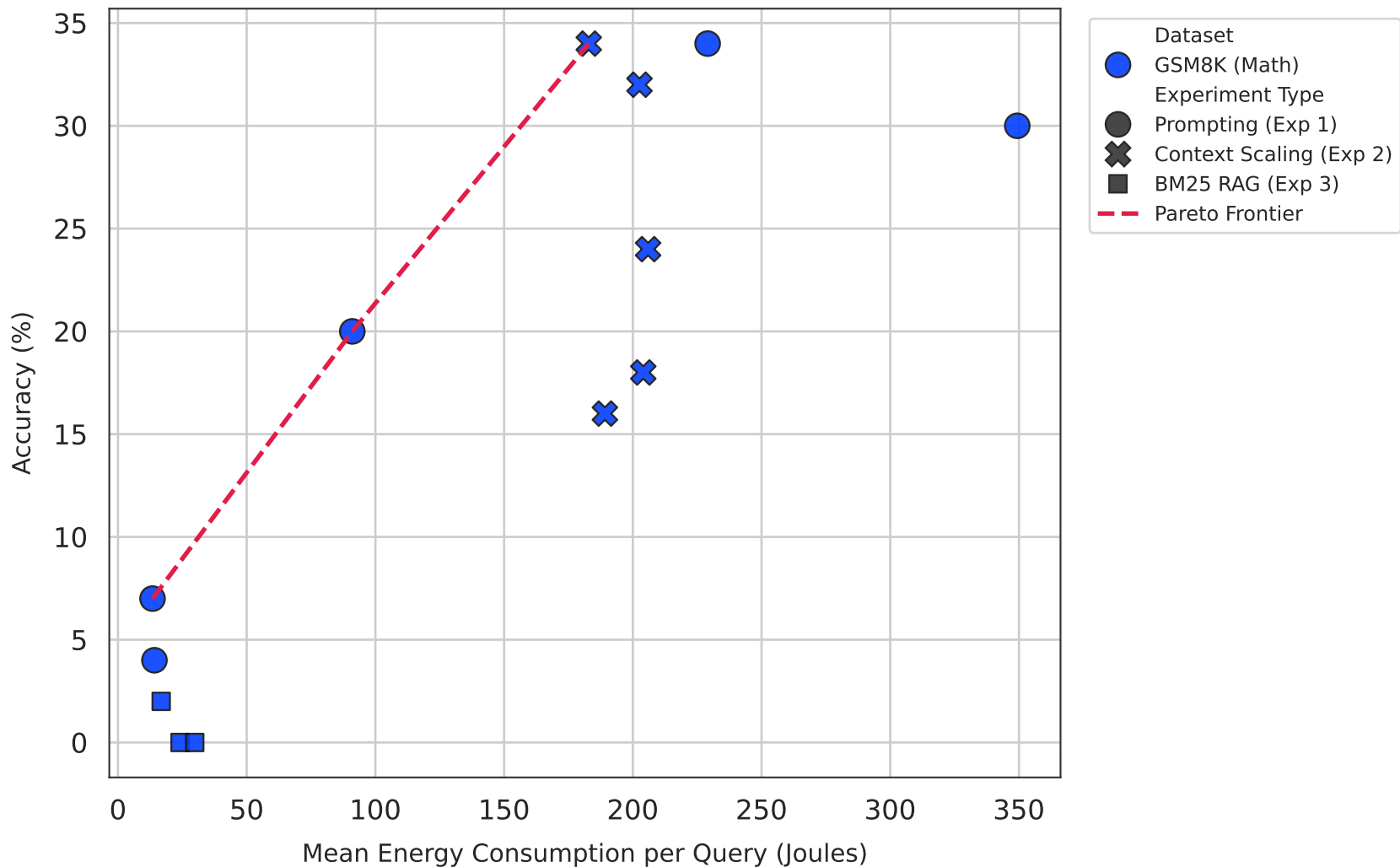
Energy vs. Accuracy Trade-Off & Pareto Frontier — gemma3:1b
