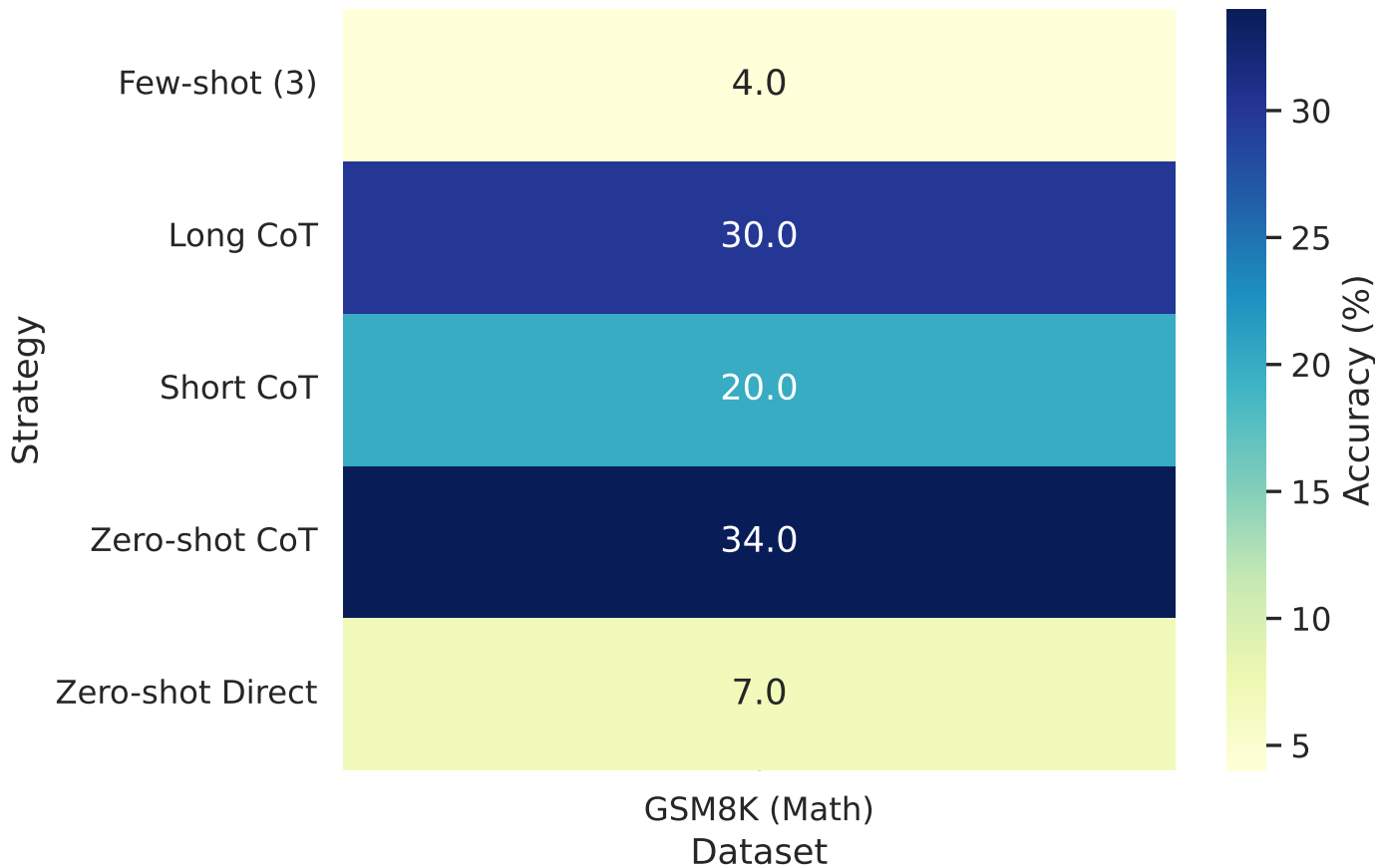
(A) Accuracy (%) by Prompting Strategy
