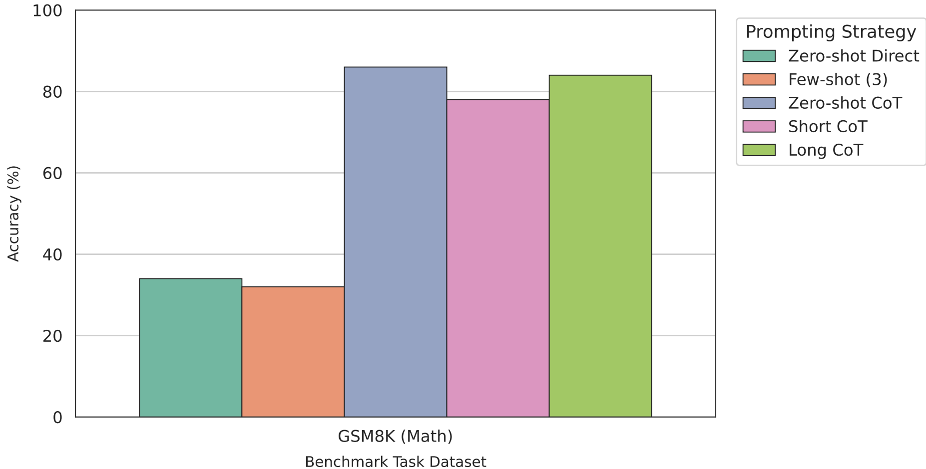
Task Accuracy by Prompting Strategy — Model: gemma3:4b (kaggle_t4_gpu)
