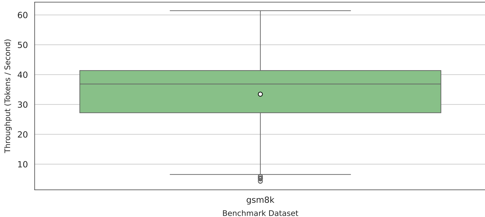
Token Generation Throughput Distribution — gemma3:4b
