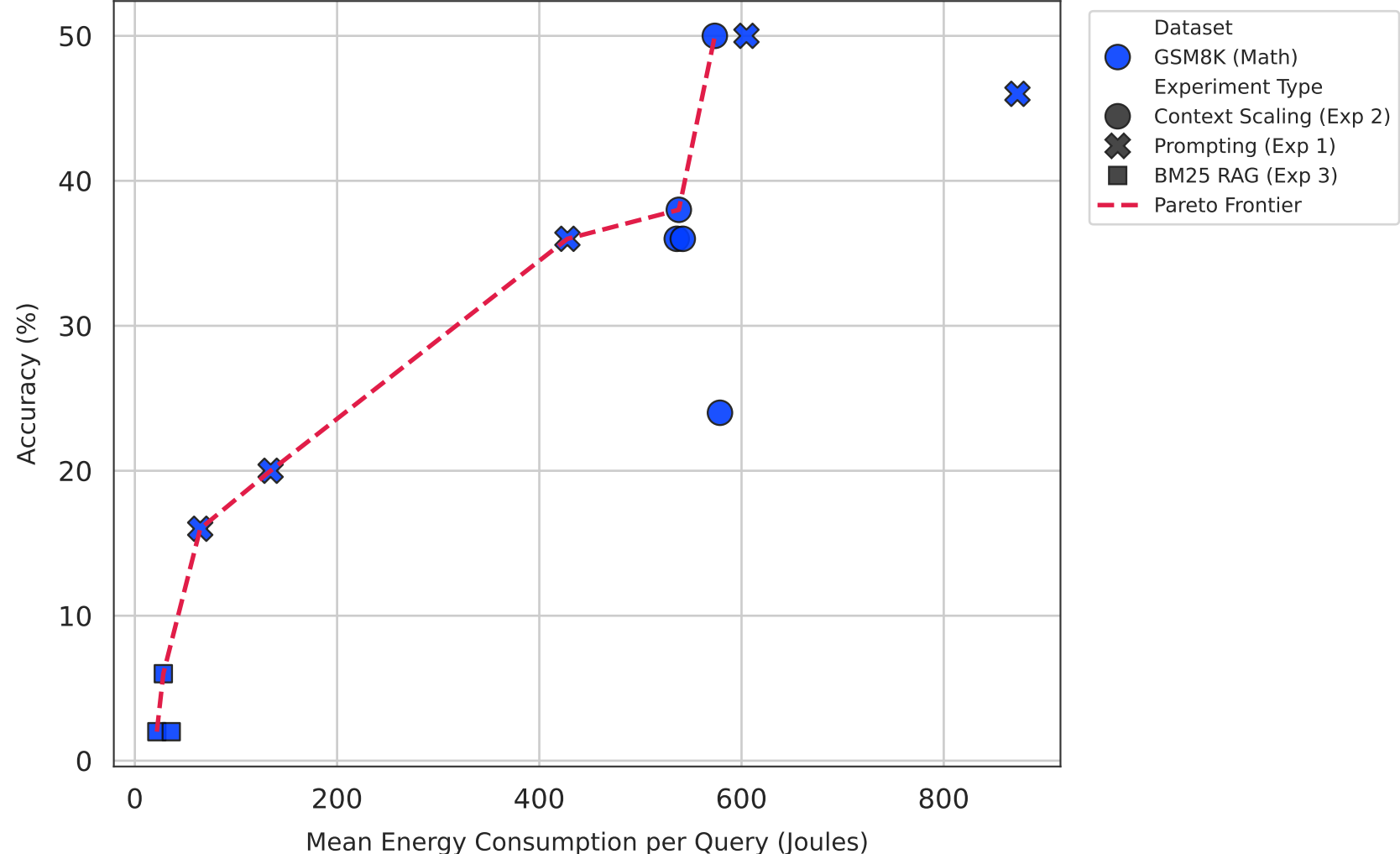
Energy vs. Accuracy Trade-Off & Pareto Frontier — qwen3.5:0.8b
