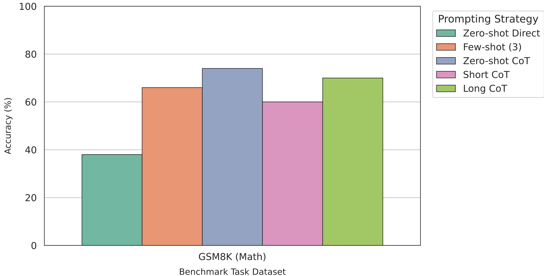
Task Accuracy by Prompting Strategy — Model: qwen3.5:2b (kaggle_t4_gpu)
