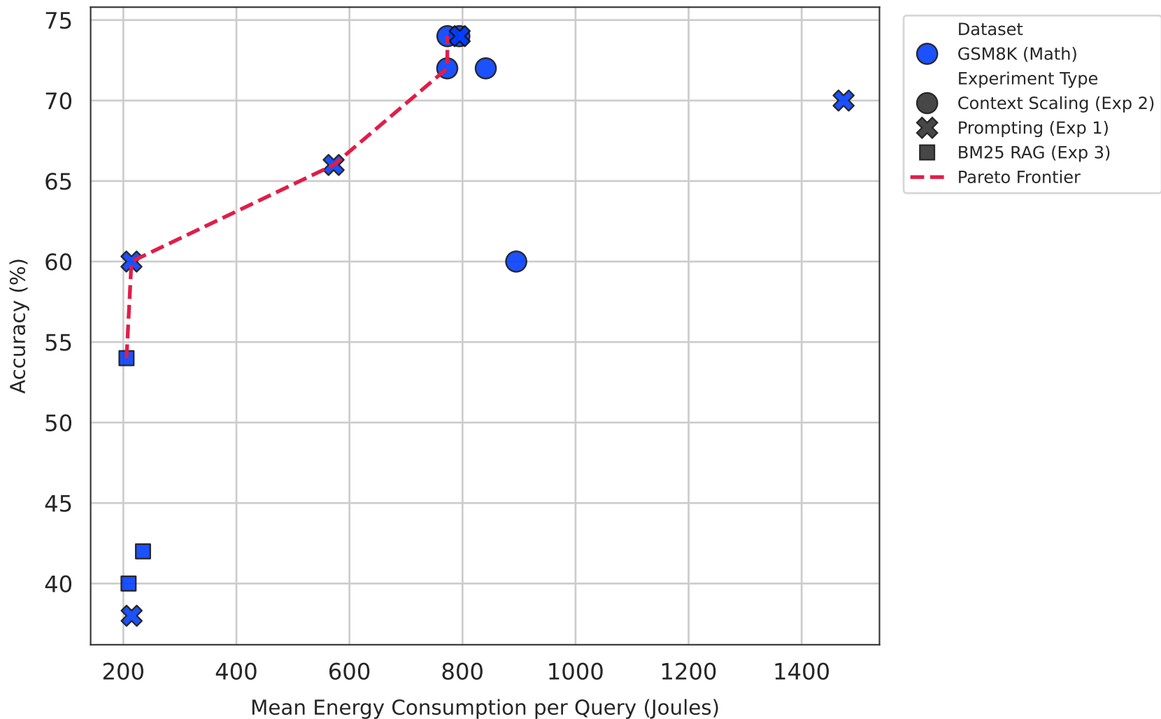
Energy vs. Accuracy Trade-Off & Pareto Frontier — qwen3.5:2b
