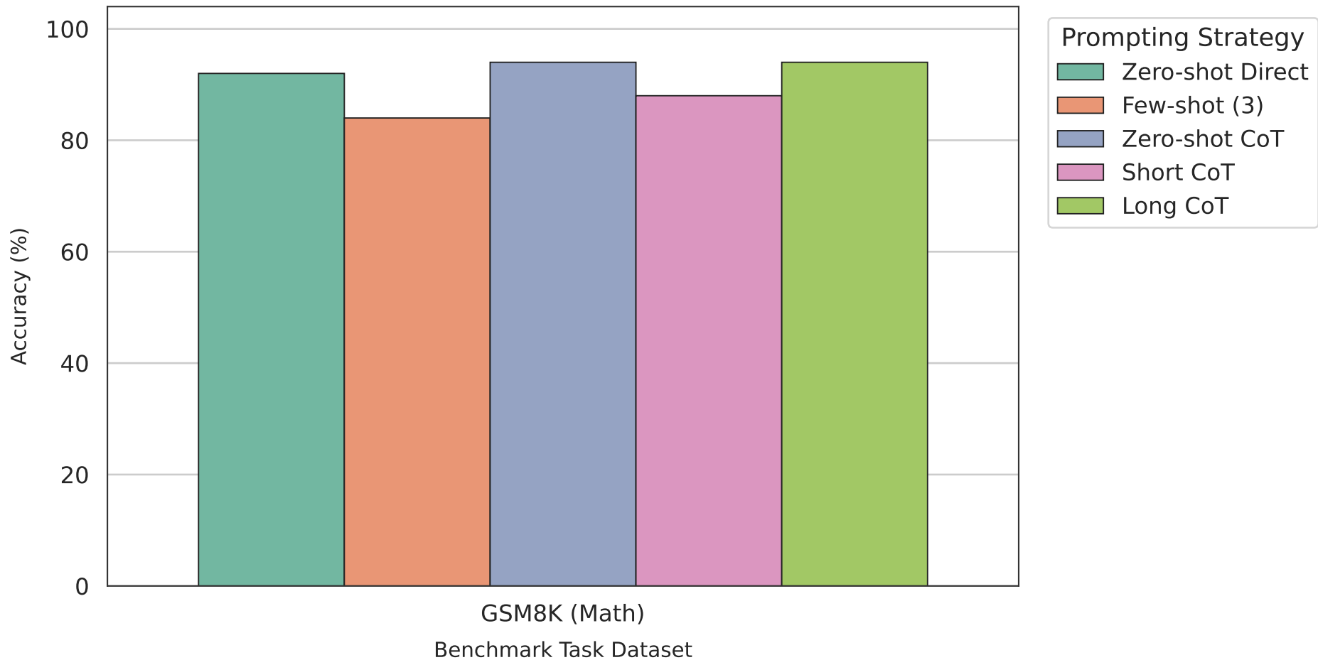
Task Accuracy by Prompting Strategy — Model: qwen3.5:9b (kaggle_t4_gpu)
