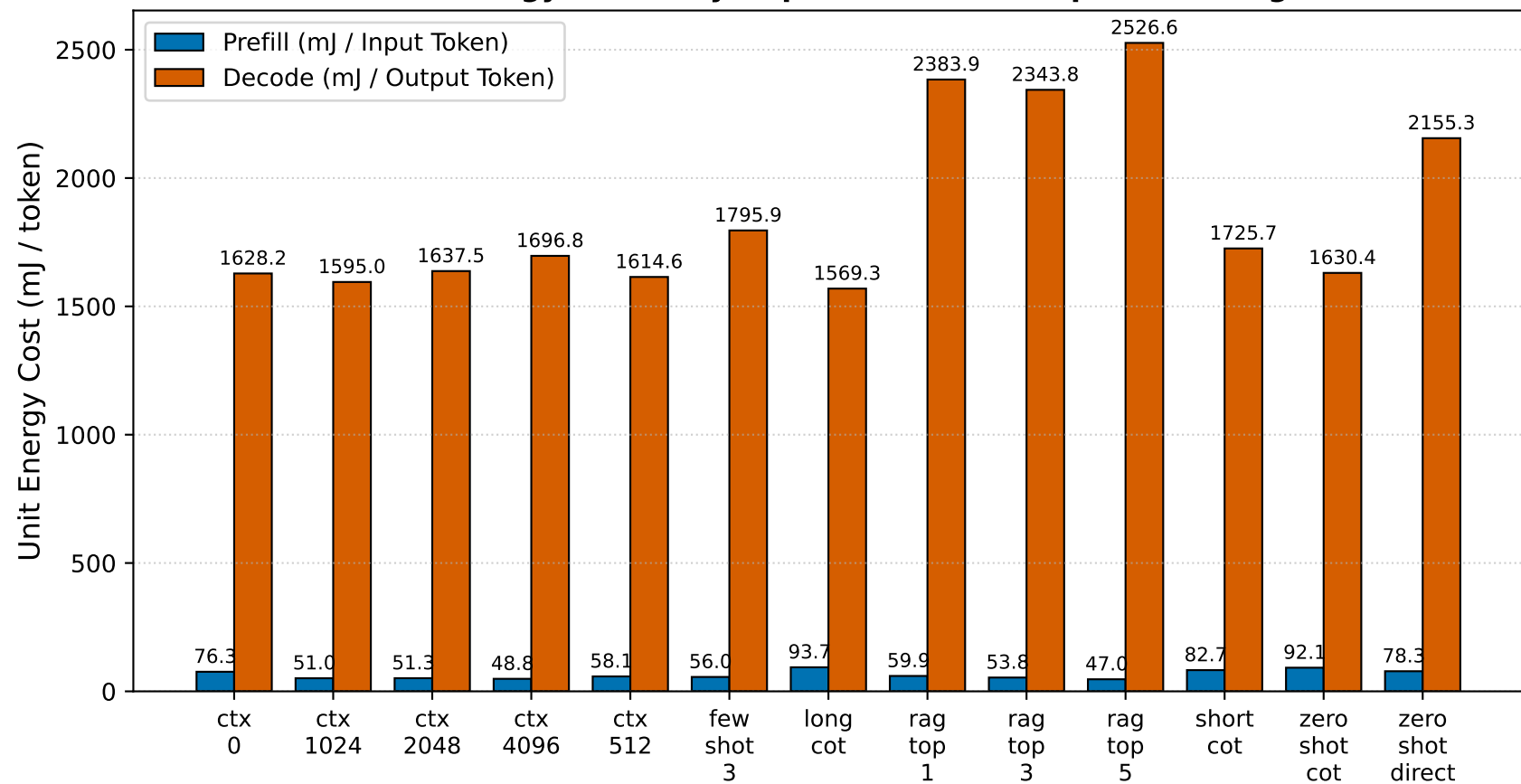
Unit Energy Efficiency: Input Prefill vs. Output Decoding
