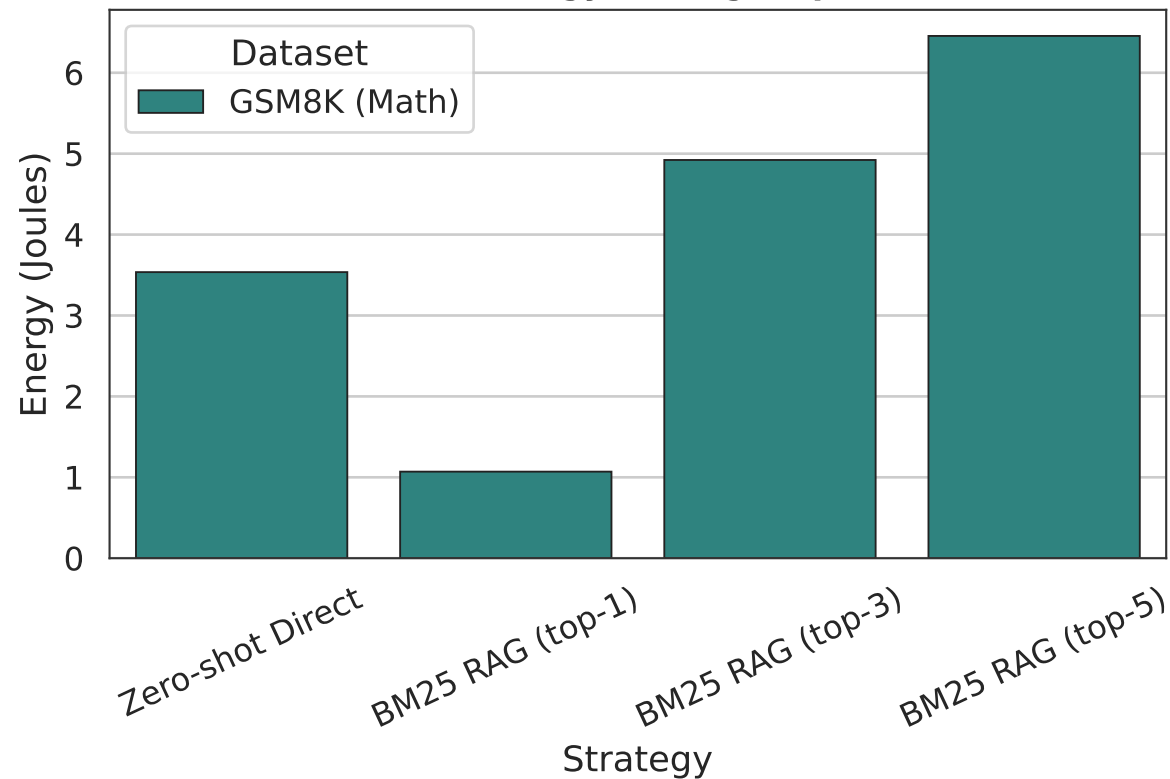
RAG Energy Scaling (Top-k)
