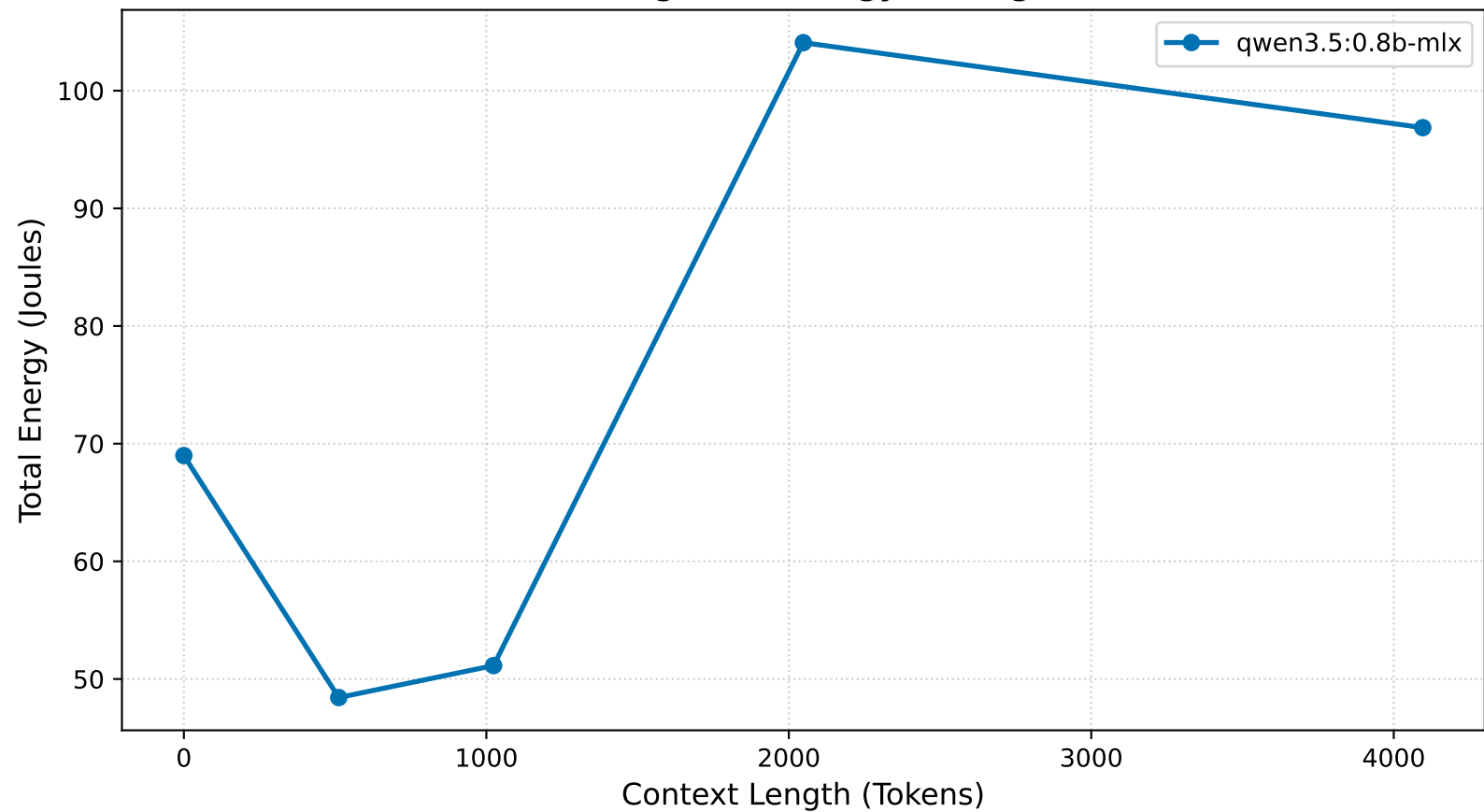
Context-Length vs. Energy Scaling Curves
