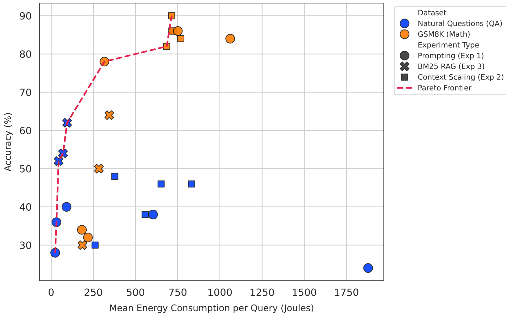
Energy vs. Accuracy Trade-Off & Pareto Frontier — gemma3:4b
