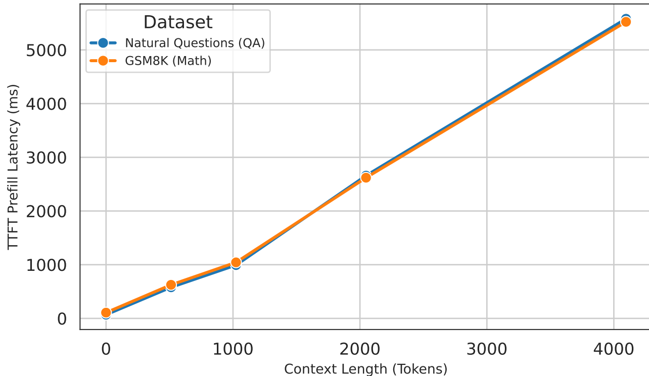
Time-to-First-Token (TTFT) vs. Context Length
