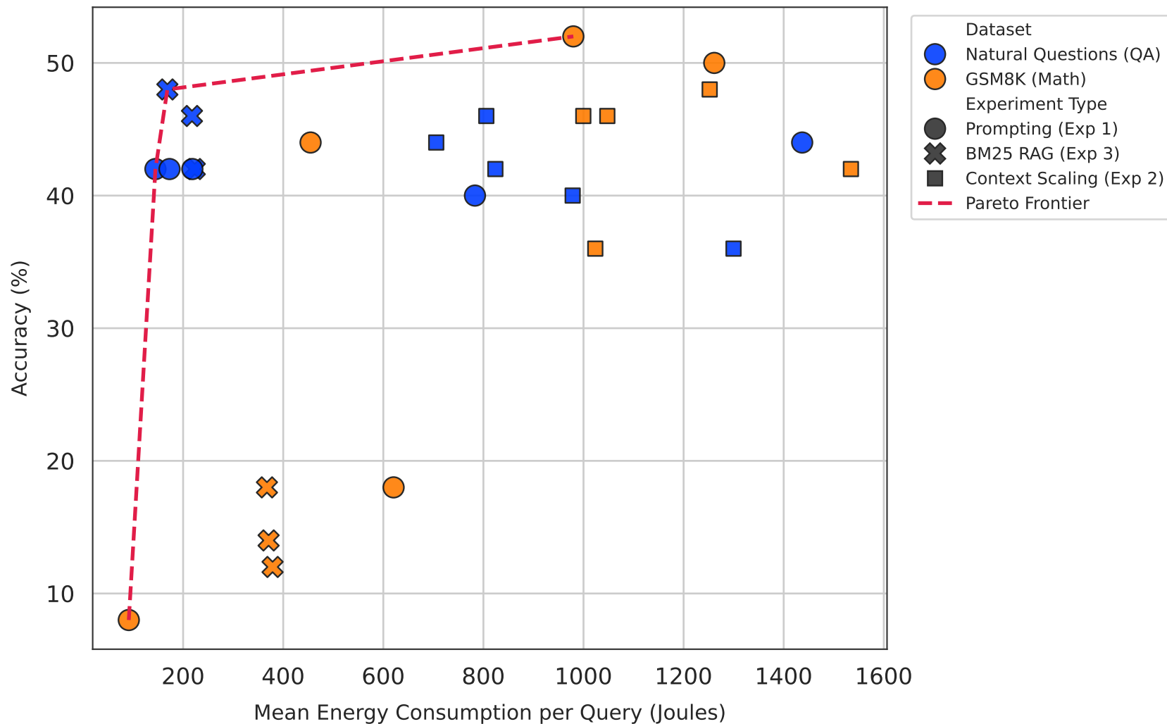
Energy vs. Accuracy Trade-Off & Pareto Frontier — mistral:7b
