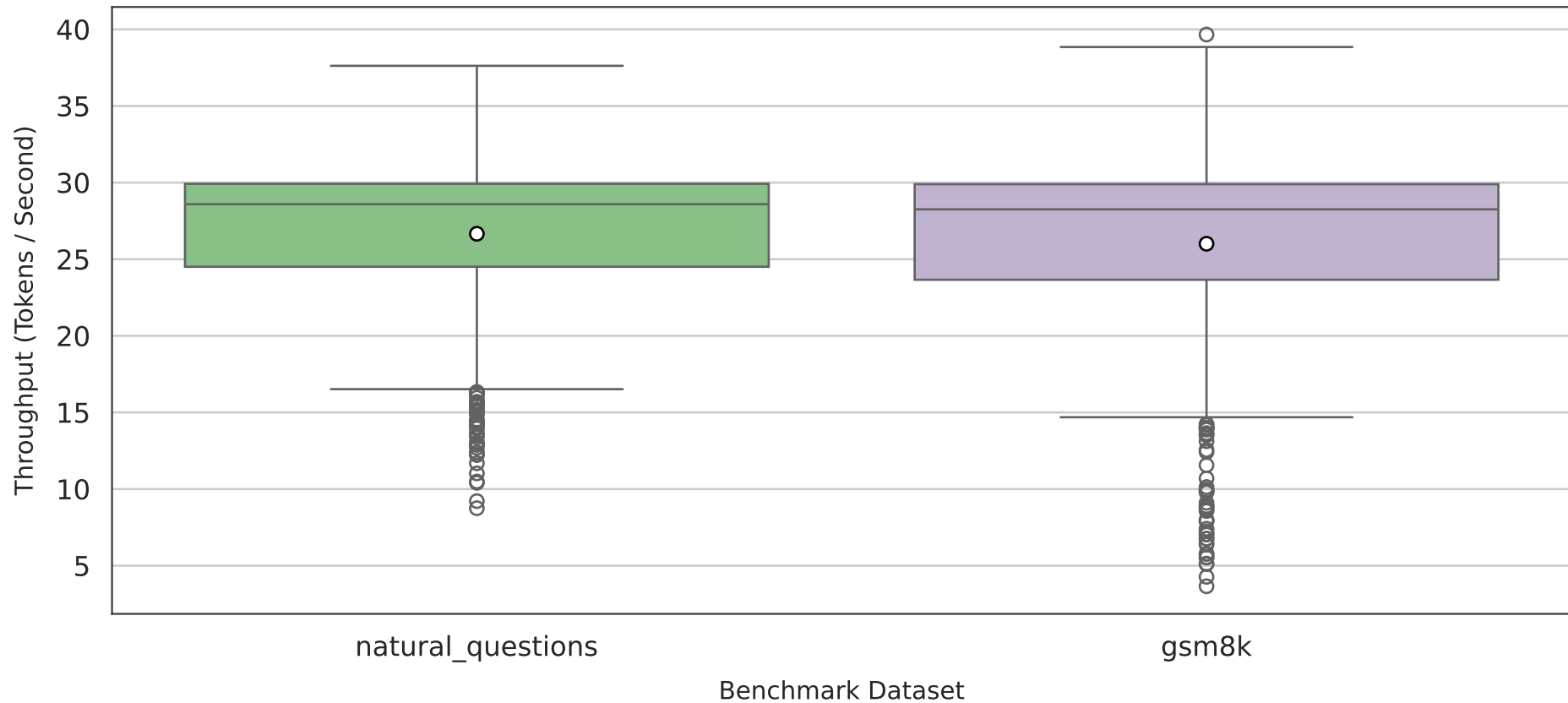
Token Generation Throughput Distribution — mistral:7b
