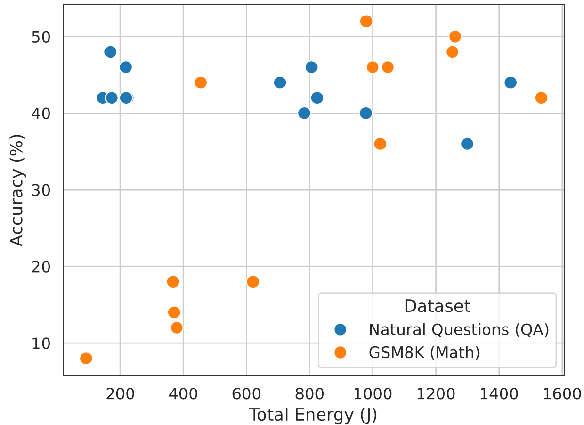
(C) Energy-Accuracy Frontier
