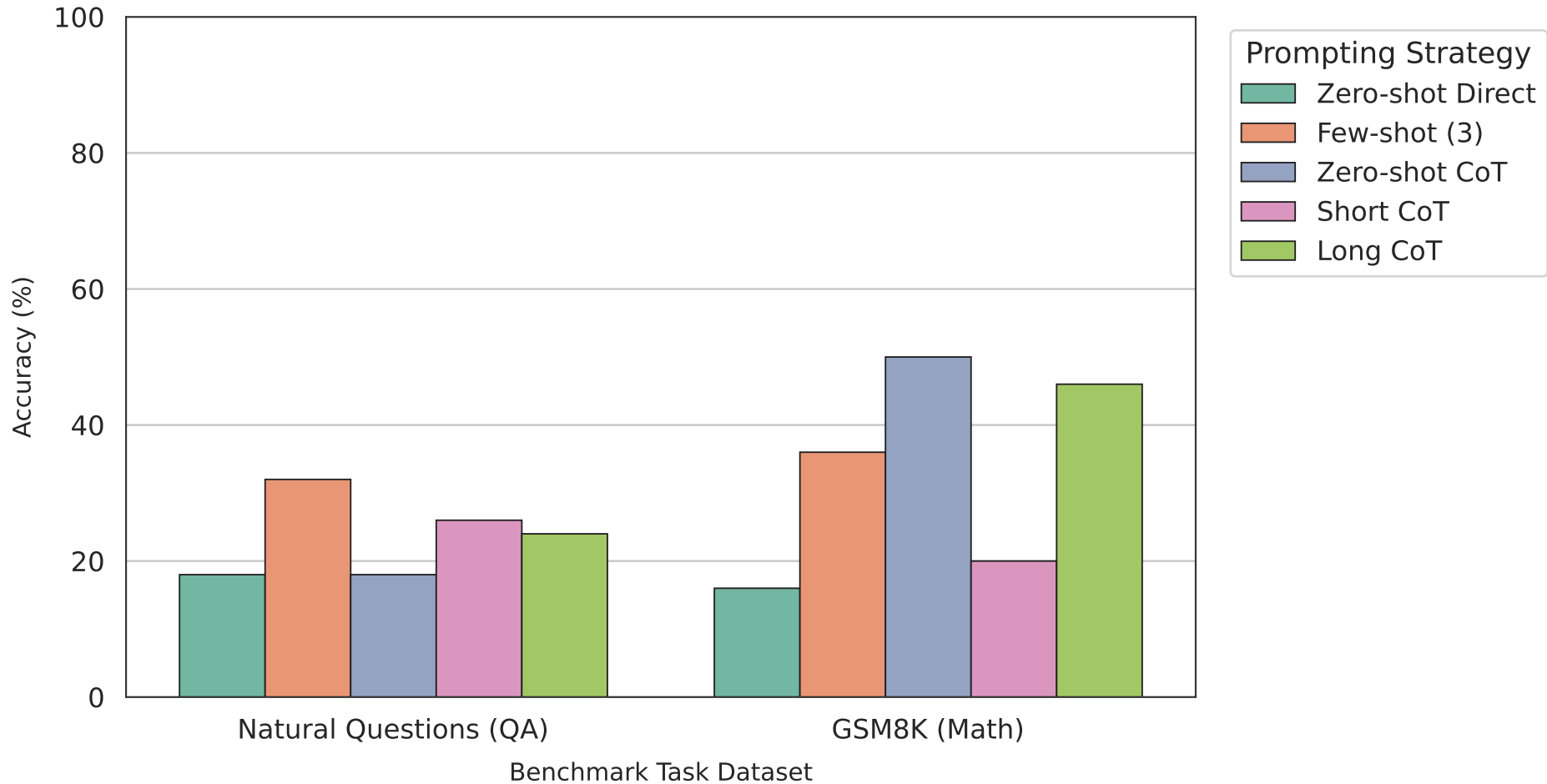
Task Accuracy by Prompting Strategy — Model: qwen3.5:0.8b (kaggle_t4_gpu)
