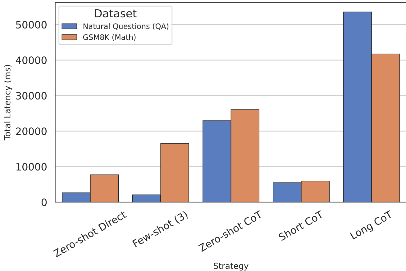
Total Latency by Prompting Strategy
