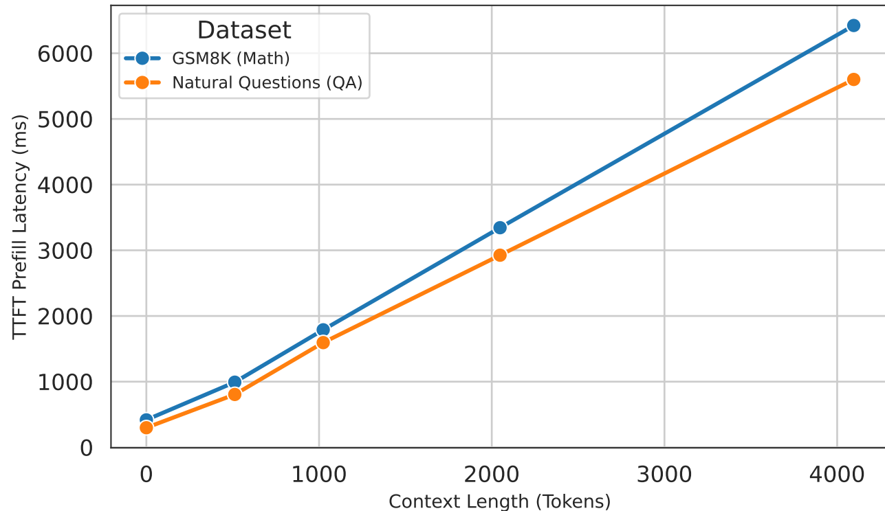
Time-to-First-Token (TTFT) vs. Context Length
