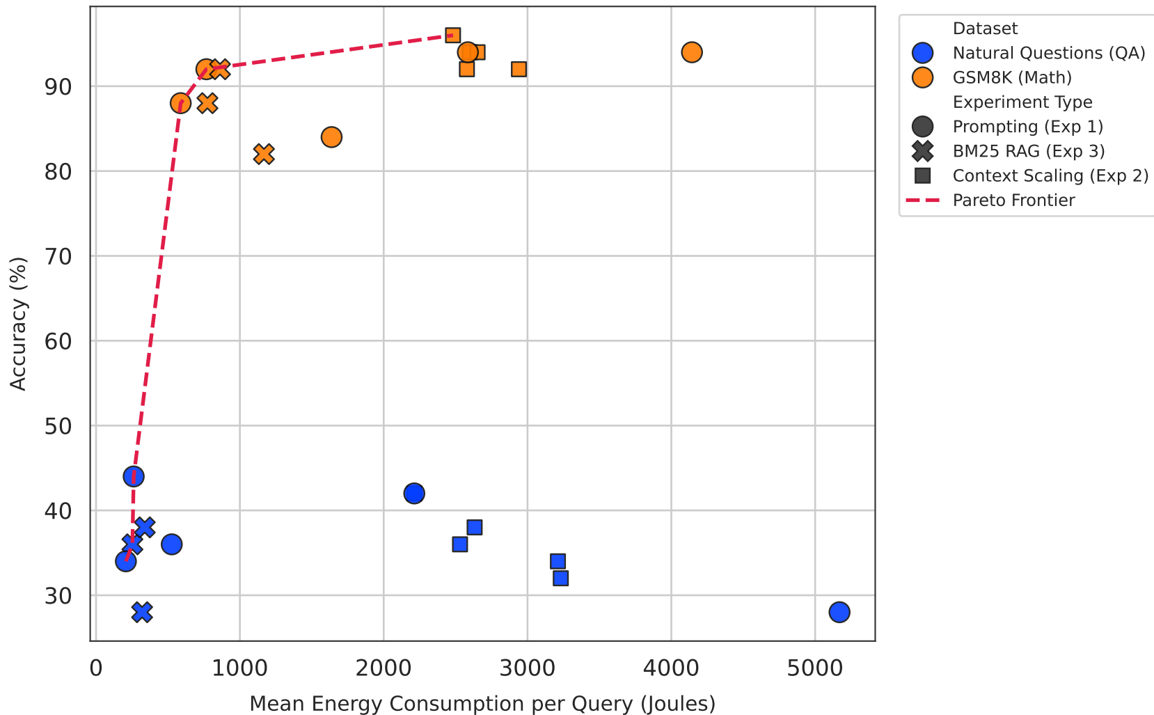
Energy vs. Accuracy Trade-Off & Pareto Frontier — qwen3.5:9b
