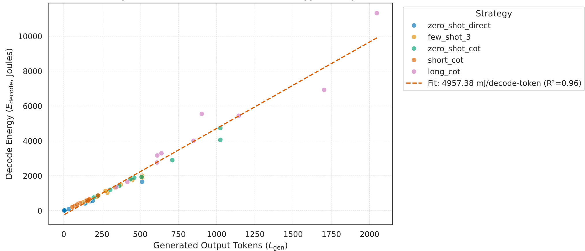
Autoregressive Generation (Decode) Energy Scaling
