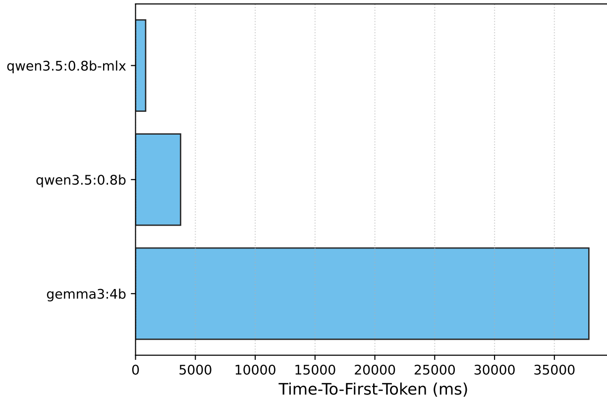
Prefill Latency (TTFT)
