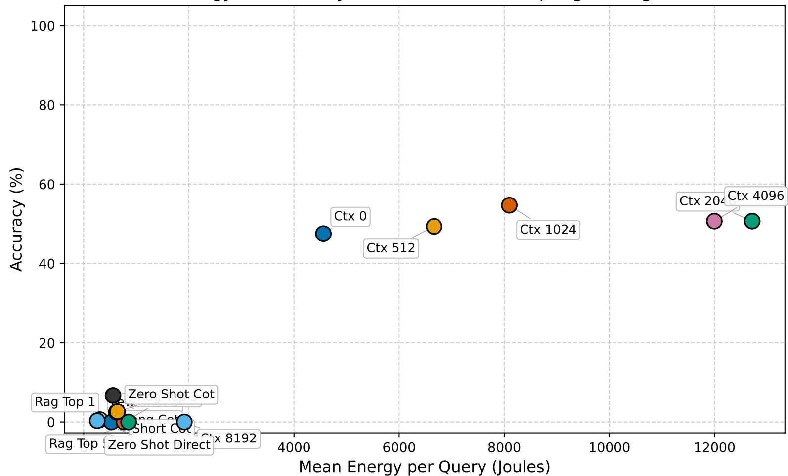
Energy vs. Accuracy Trade-off Across Prompting Strategies
