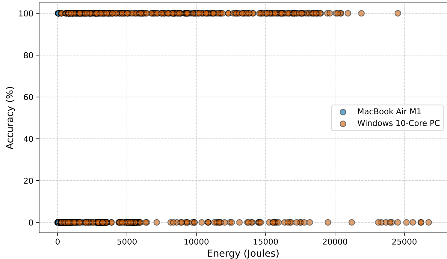
Cross-Hardware Energy vs. Accuracy Distribution
