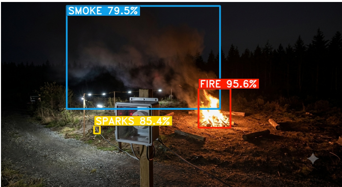
AI DETECTION RESULT (ACTUAL BOUNDING BOXES)
