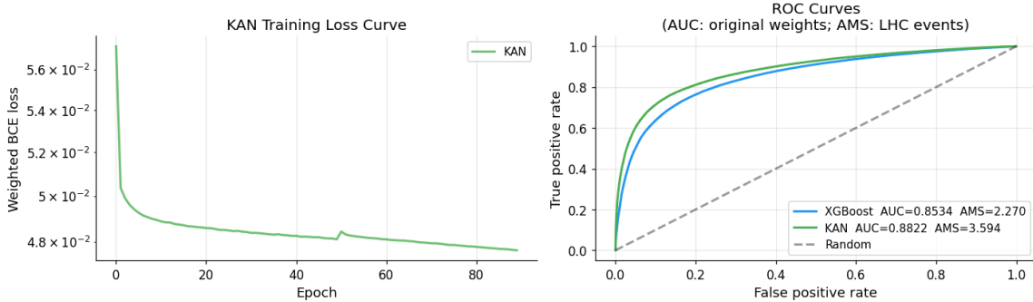
Figure 1: Left: KAN training loss converging. Right: ROC curves, where the tuned KAN (AUC 0.882) lies above XGBoost (AUC 0.853).
