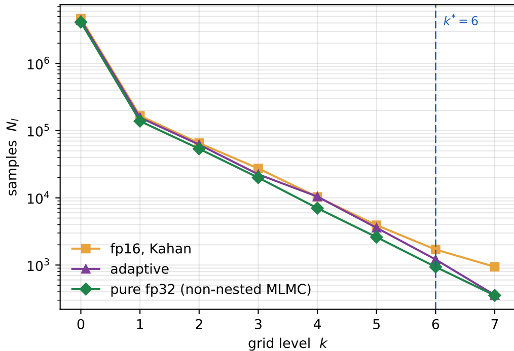
Milstein correction
